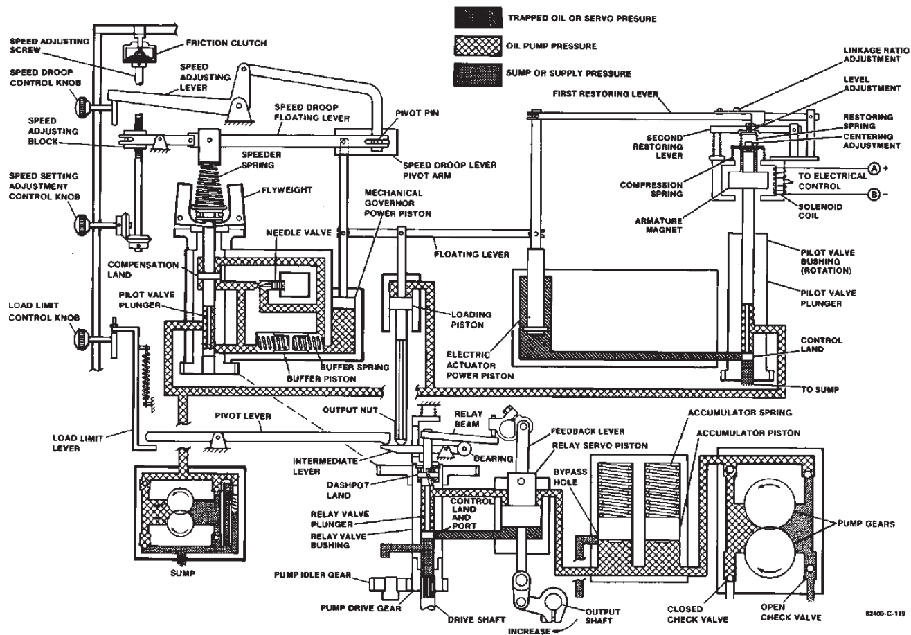
SCHEMATIC DIAGRAM EGB-29P/58P GOVERNOR/ACTUATOR
